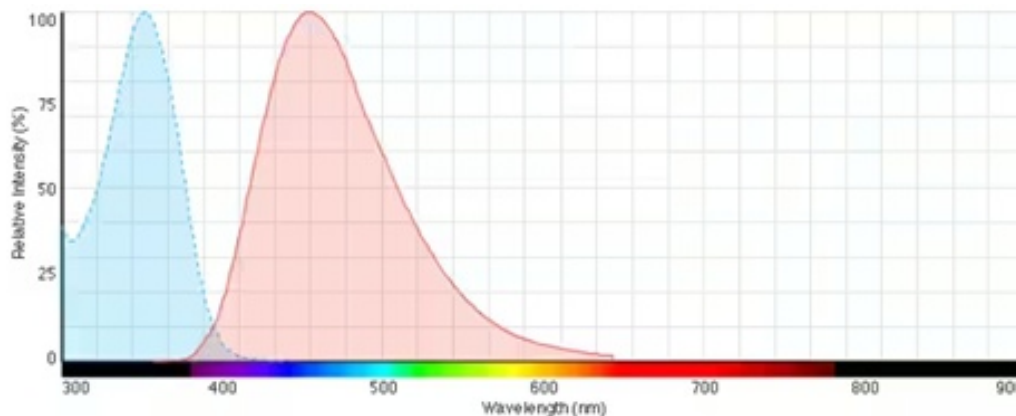
Fig. Fluorescence excitation and emission spectra of Hoechst 33342 bound to DNA
